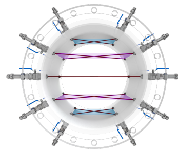
Wetted sensors arranged in five parallel planes
