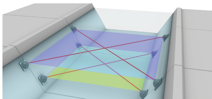
Multi-path Kanalıs system with crossed paths in two planes
