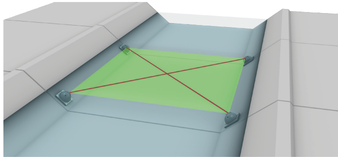
Crossed-path Kanalıs system in irrigation channel
